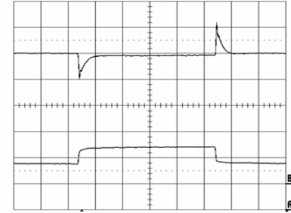
Output voltage response to load current step- change (13-26-13 A) at: T_{ref} = +25^\circ\text{C} , V_i = 12.0\text{ V} . Top trace: output voltage (100mV/div.). Bottom trace: load current (20 A/div.). Time scale: 0.1 ms/div.
