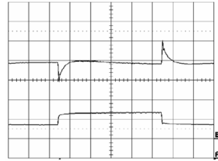
Output voltage response to load current step- change (13-26-13 A) at: T_{ref} = +25^{\circ}C , V_i = 12.0 V. Top trace: output voltage (100mV/div.). Bottom trace: load current (20 A/div.). Time scale: 0.1 ms/div.
