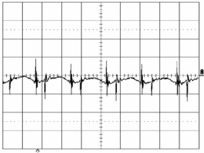
Output voltage ripple (20mV/div.) at: T_{ref} = +25^\circ\text{C} , I_O = 26\text{ A} resistive load, V_i = 12.0\text{ V} . Time scale: 1 \mu\text{s} /div. See the filter in the Output ripple and noise section (EMC Specification).
