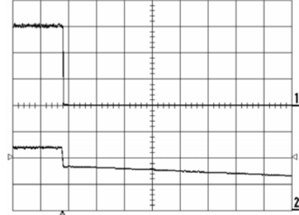
Shut-down enabled by disconnecting V_i at: T_{ref} = +25^\circ\text{C} , I_O = 26\text{ A} resistive load, V_i = 12.0\text{ V} . Top trace: output voltage (0.5 V/div.). Bottom trace: input voltage (5 V/div.). Time scale: 10.0 ms/div.
