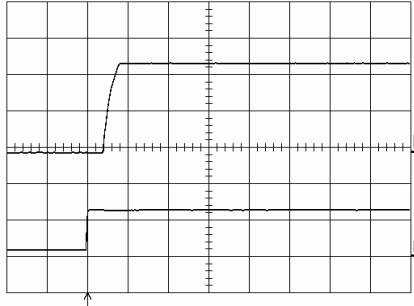
Start-up enabled by connecting V_i at: T_{ref} = +25^\circ\text{C} , I_O = 26\text{ A} resistive load, V_i = 12.0\text{ V} . Top trace: output voltage (2.0 V/div.). Bottom trace: input voltage (10 V/div.). Time scale: 10 ms/div.
