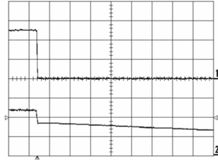
Shut-down enabled by disconnecting V_i at: T_{ref} = +25^\circ\text{C} , I_O = 26\text{ A} resistive load, V_i = 12.0\text{ V} . Top trace: output voltage (2.0 V/div.). Bottom trace: input voltage (5 V/div.). Time scale: 10.0 ms/div.
