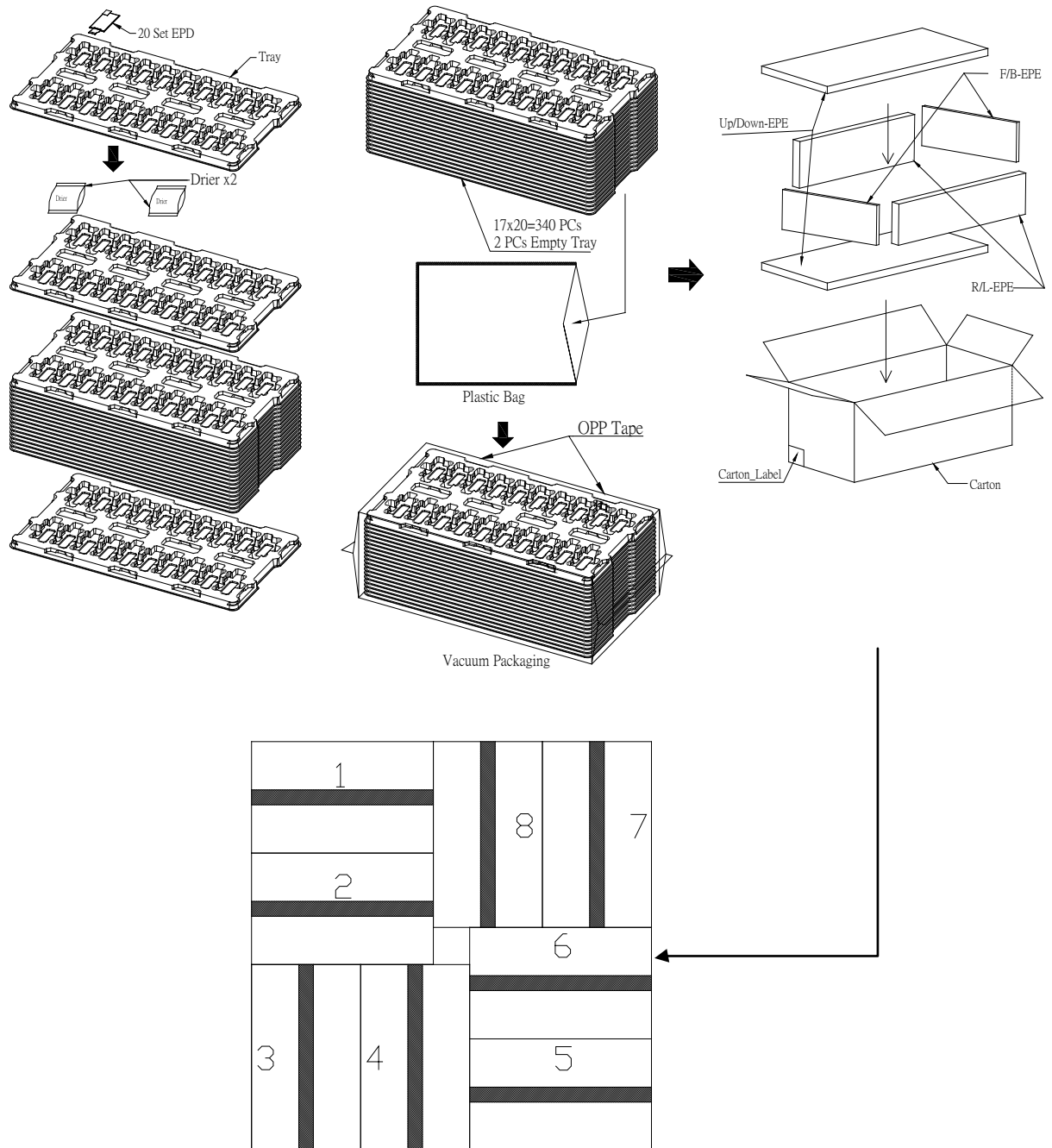
Figure 7-1 Packing Diagram
