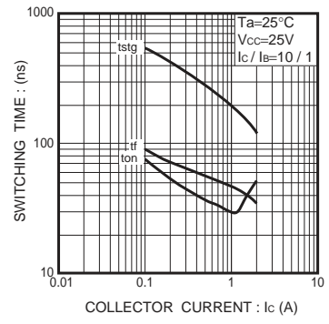
Fig.9 Switching Time
