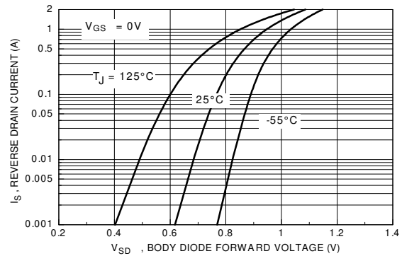
Figure 8. Body Diode Forward Voltage Variation with Reverse Drain Current
