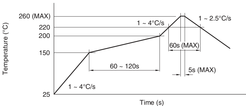
Fig. 19 Temperature Profile
