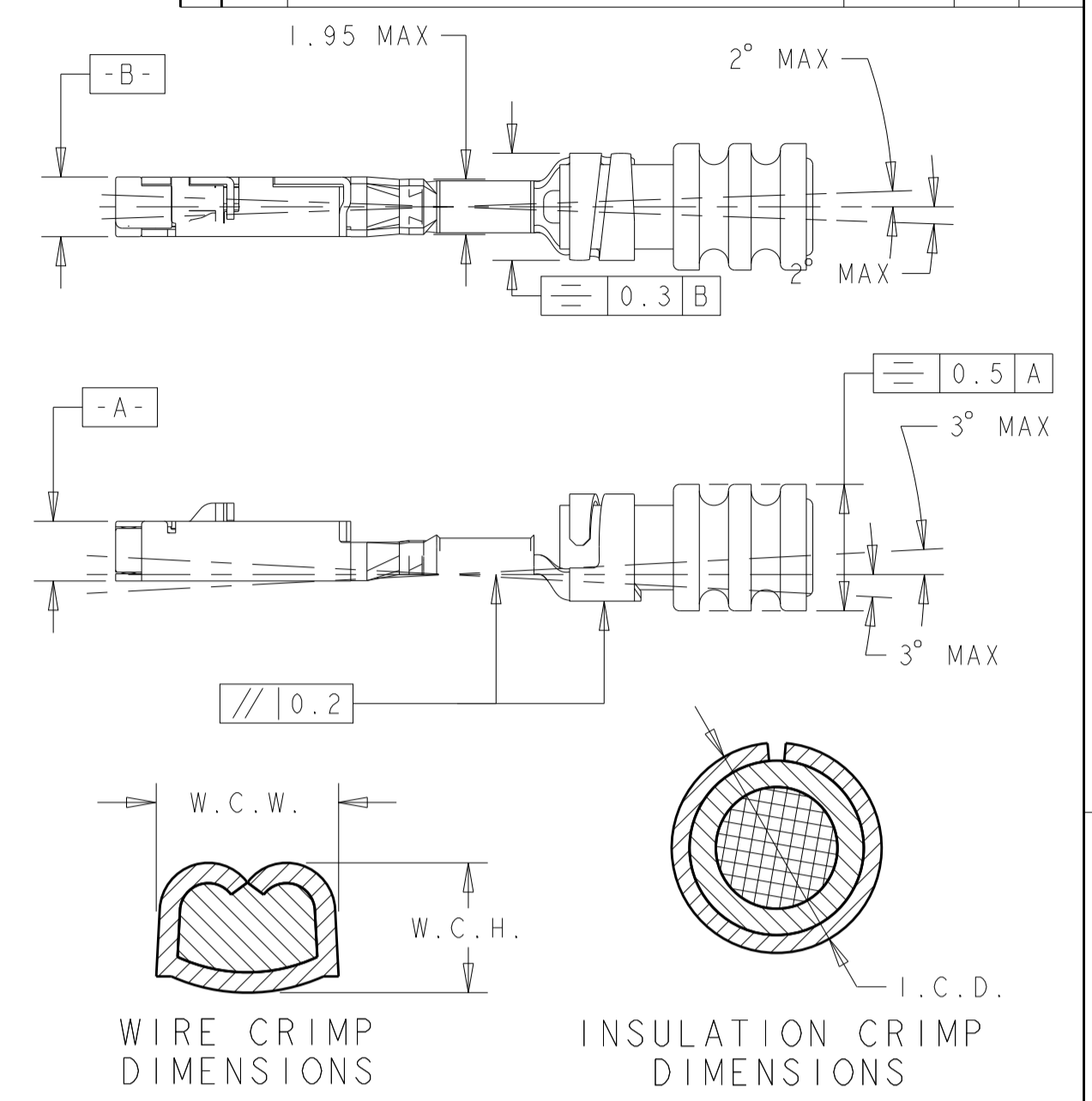
SECTION A-A SECTION A-A SHOWN WITH TPA IN ITS LATCHED POSITION FOR REFERENCE ONLY
