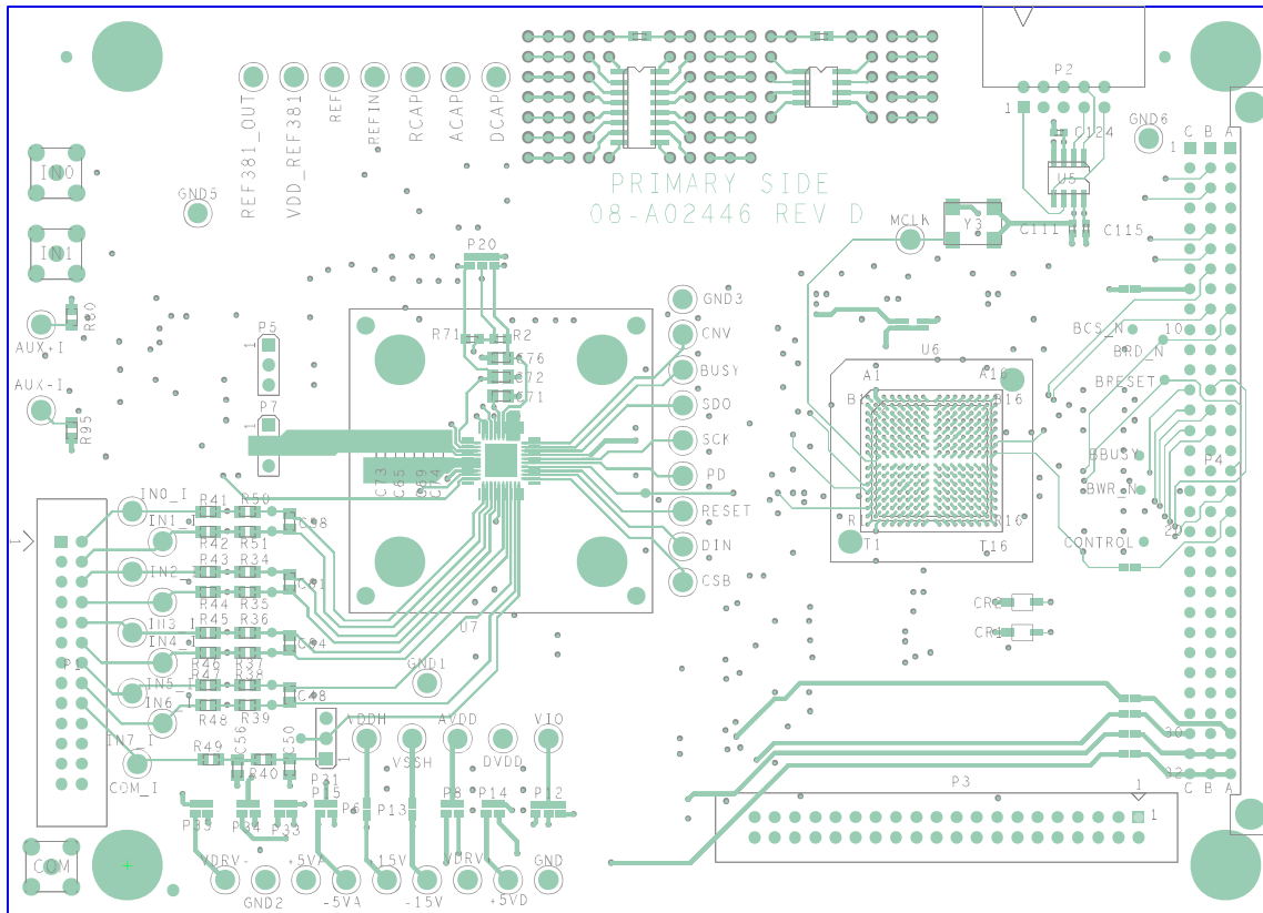
Figure 32. Silkscreen, Top
