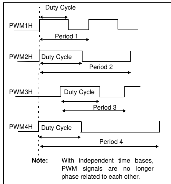
FIGURE 12-11: INDEPENDENT TIME BASE PWM
