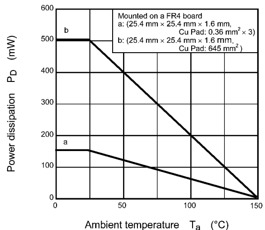
Fig. 7.12 P_D - T_a
