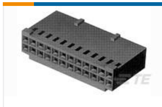
TE Part #3-87977-4 18 MODIV HSG COMP DR .100 POL
