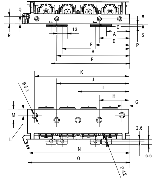
Screw Termination
