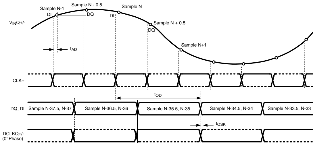
Figure 3. Clocking in 1:4 Demux DES Mode*
