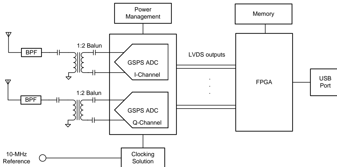
Figure 72. Simplified Schematic
