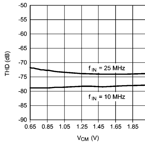
THD vs. V_{CM}
