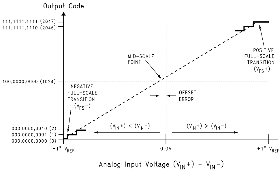
FIGURE 1. Transfer Characteristic
