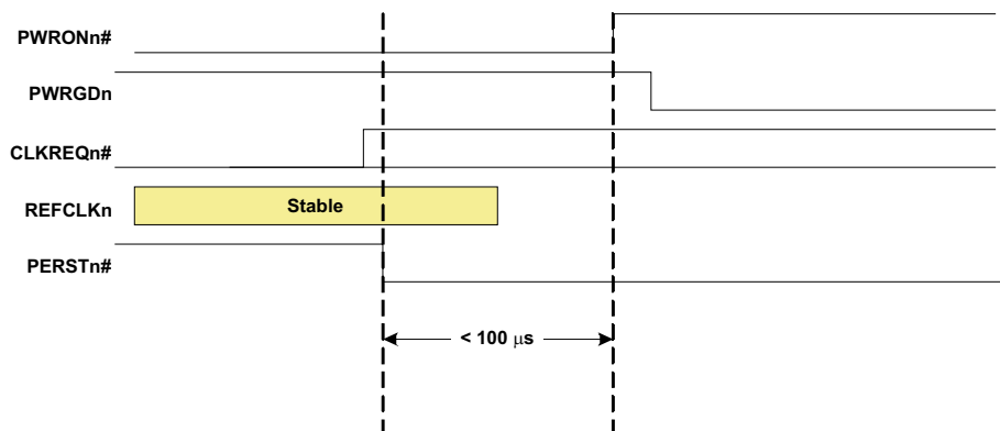
Figure 5-4. Normal Power-Down
