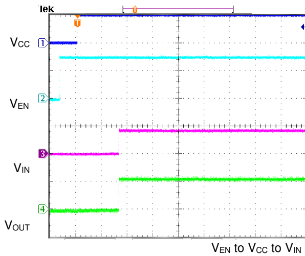
Figure 19. Input Sequence
