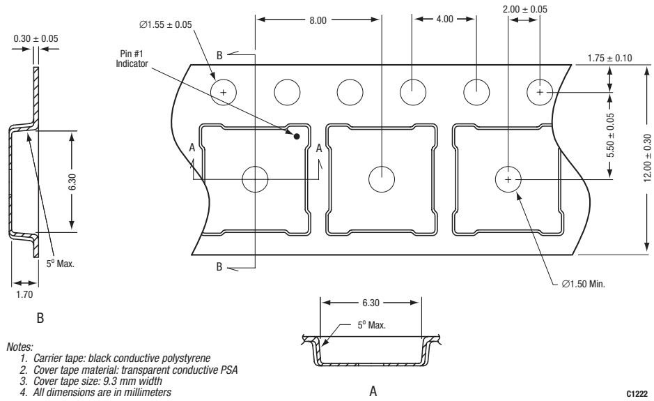
Figure 41. SKY73021 Tape and Reel Dimensions
