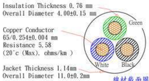
線材截面圖 (Wire Cross-Section)
