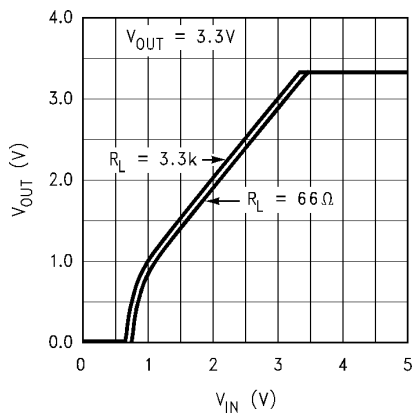
Dropout Characteristics
