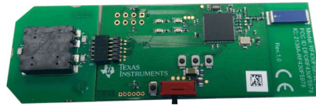
Figure 23. RF430F5978EVM Photo
