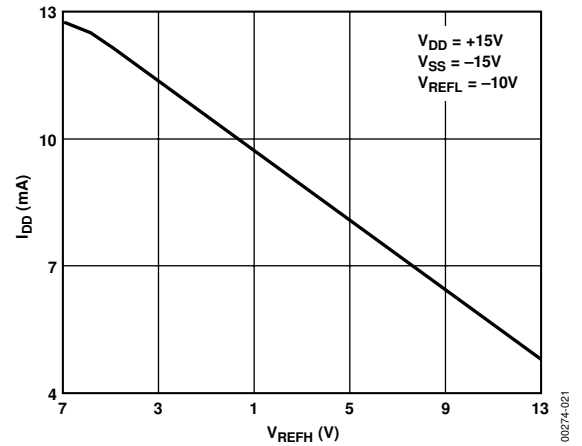
Figure 20. I_{DD} vs. V_{REFH} (All DACs High)
