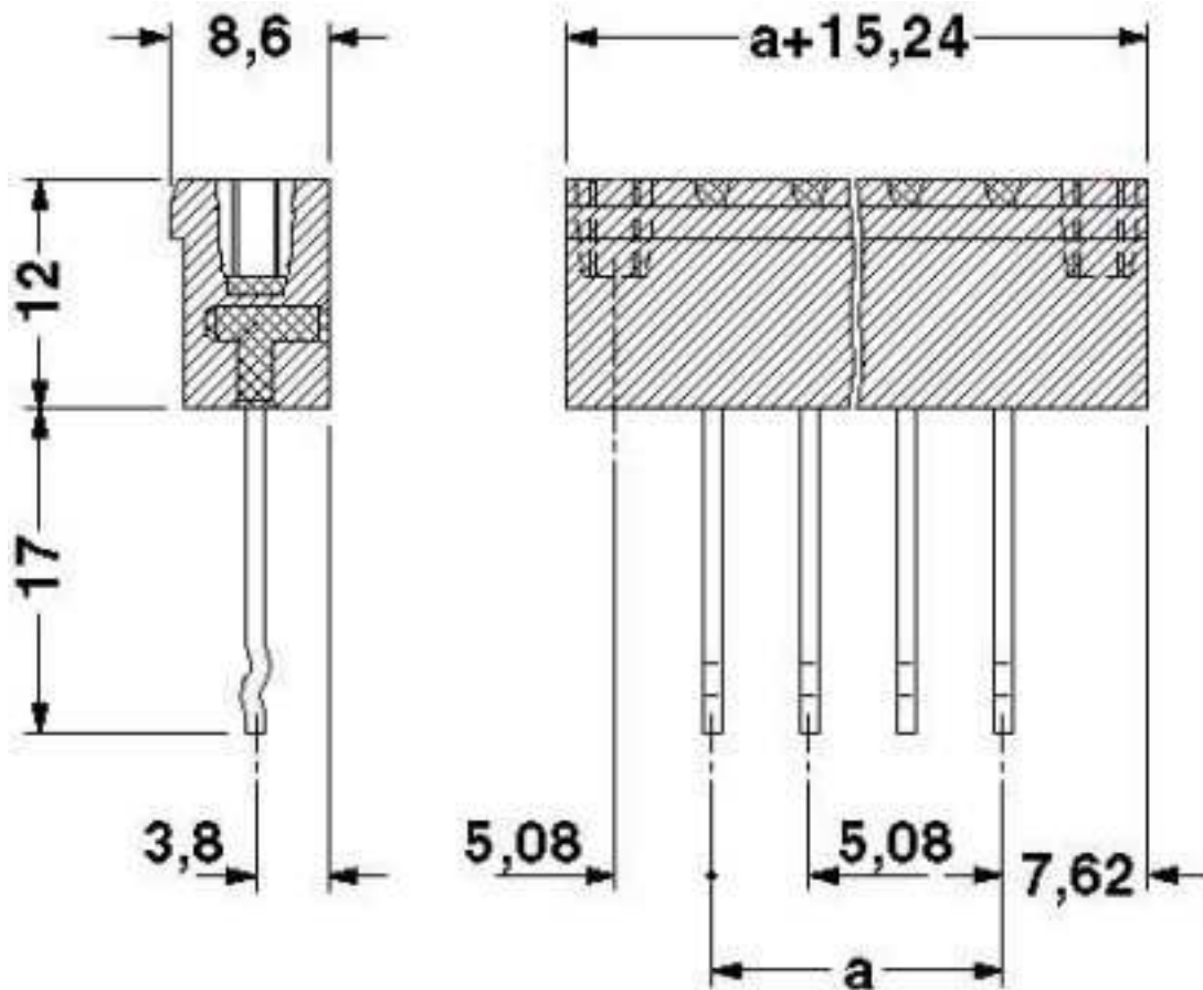
Dimensioned drawing
