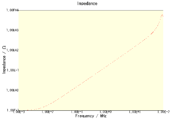
CLF12555T-2R2N-CA
