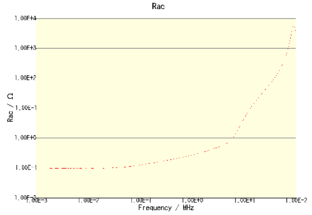
CLF12555T-2R2N-CA
