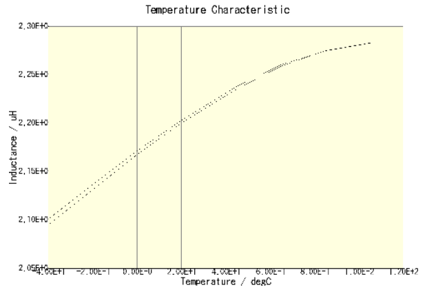
CLF12555T-2R2N-CA(DC = 0A)
