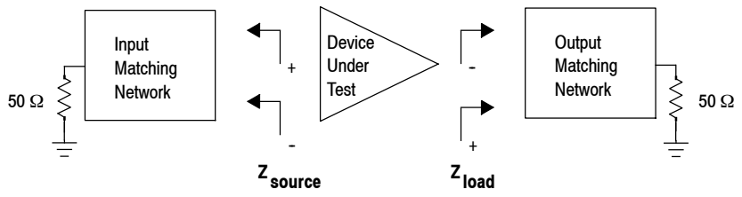
Figure 20. Broadband Series Equivalent Source and Load Impedance — 87.5–108 MHz
