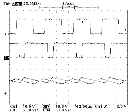
Figure 5 - Ch1: Gate signal for sync FET (master, pin-14). Ch2: Gate signal for sync FET (slave, pin-11). Ch3: Inductor current for master channel (L3). Ch4: Inductor current for slave channel (L4). V_{MASTER}=5V , V_{SLAVE}=12V , I_{OUT}=10A
