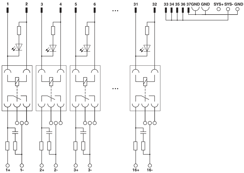
Circuit diagram
