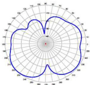
ELEVATION @ 750 MHz
