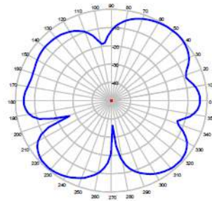
ELEVATION @ 950 MHz
