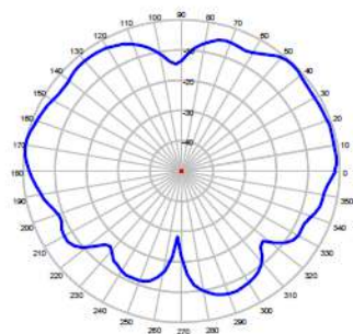
ELEVATION @ 2650 MHz
