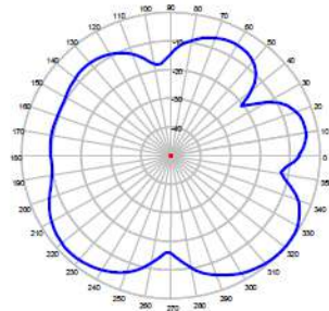
ELEVATION @ 850 MHz
