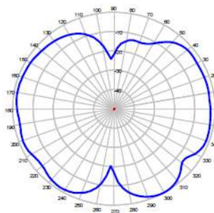
ELEVATION @ 1710 MHz
