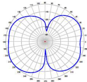
ELEVATION @ 694 MHz
