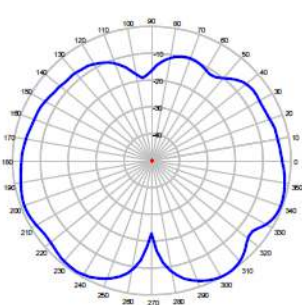
ELEVATION @ 1880 MHz
