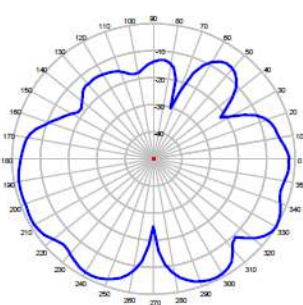
ELEVATION @ 2150 MHz
