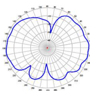
ELEVATION @ 2450 MHz
