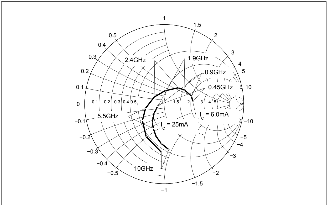
Figure 15 Source impedance for minimum noise figure Z_{opt} = f(f) , V_{CE} = 3 V, I_C = 6 / 25 mA
