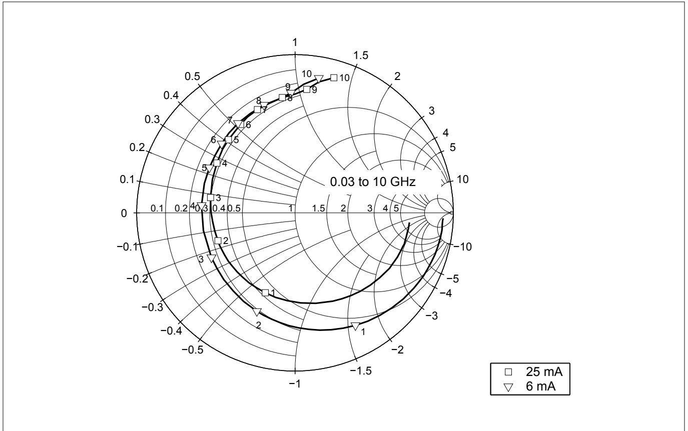
Figure 14 Input reflection coefficient S_{11} = f(f) , V_{CE} = 3 V, I_C = 6 / 25 mA
