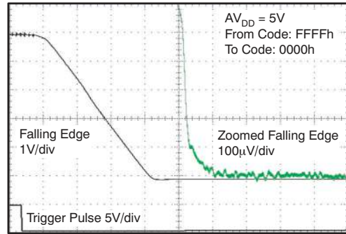
Figure 28. Full-Scale Settling Time 5-V Falling Edge
