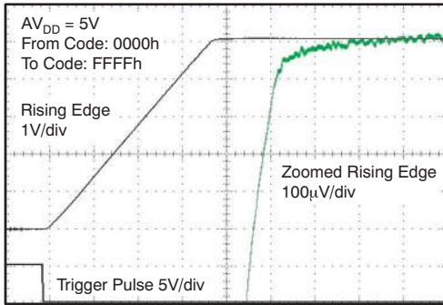
Figure 27. Full-Scale Settling Time 5-V Rising Edge
