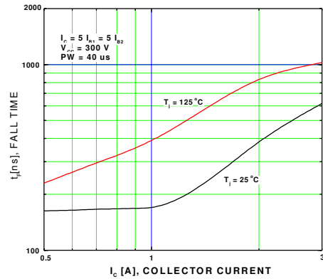
Figure 18. Resistive Switching Time, t_{fri}
