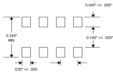
PAD LAYOUT
