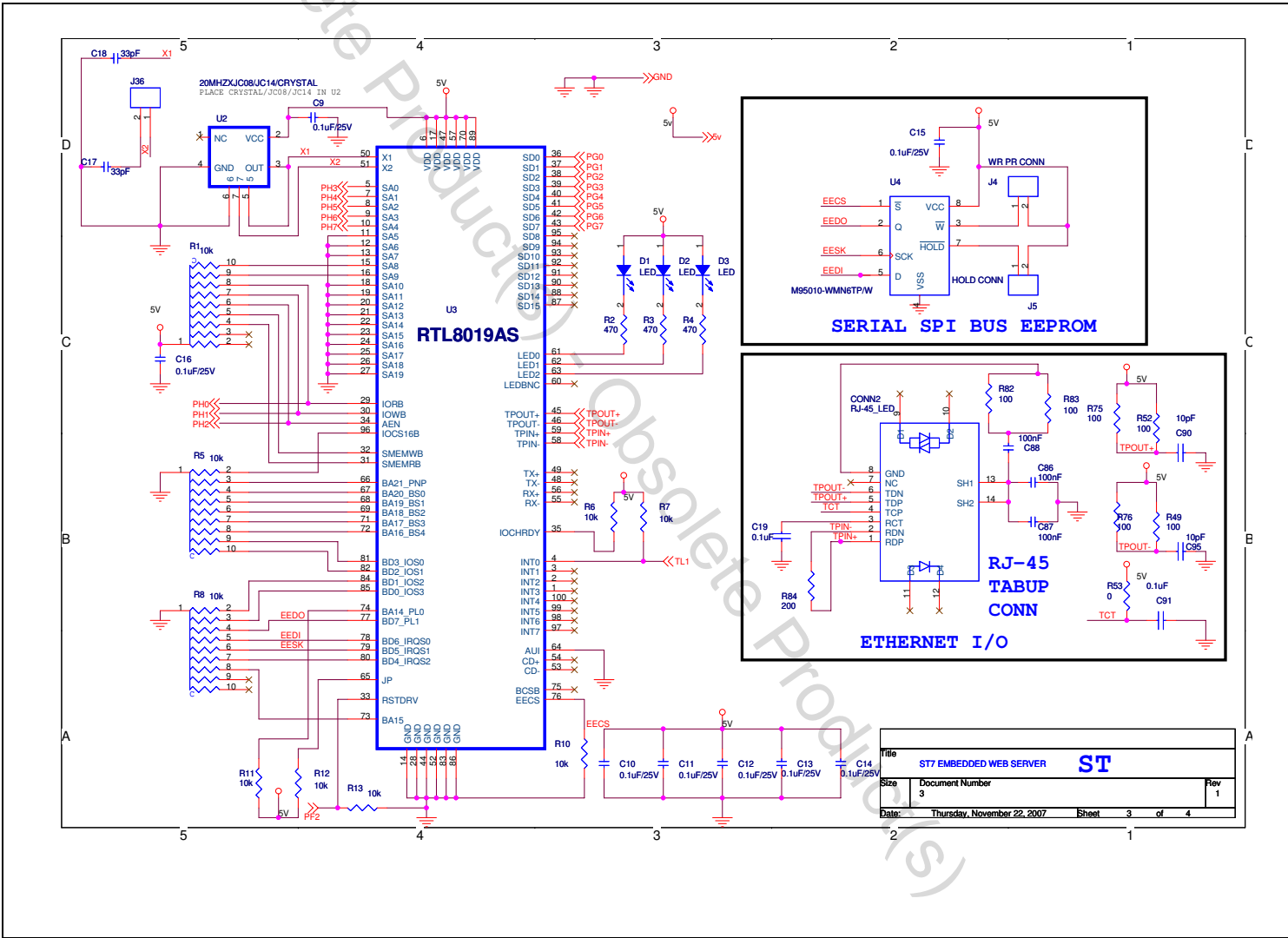
Figure 3. Ethernet
