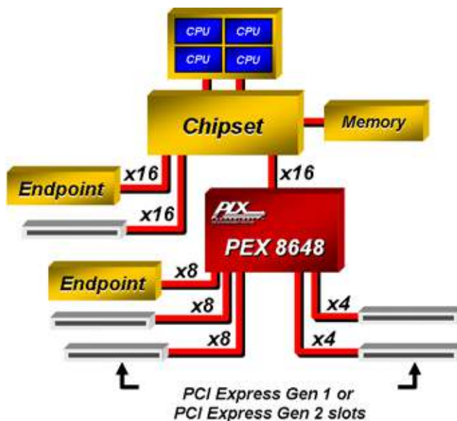
Figure 2-3. Fan-In/Fan-Out Usage
