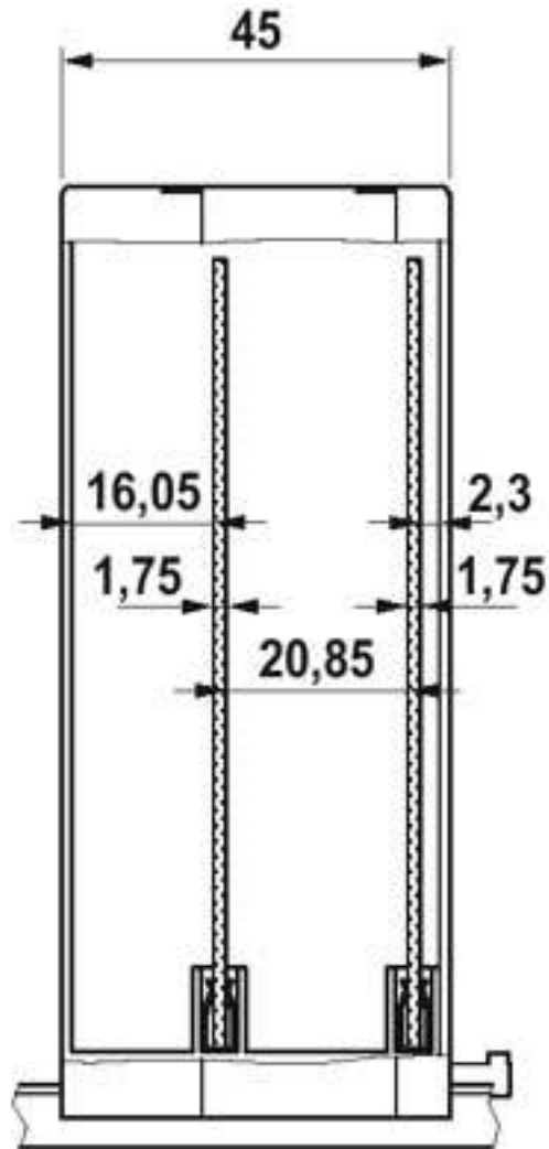
Dimensioned drawing
