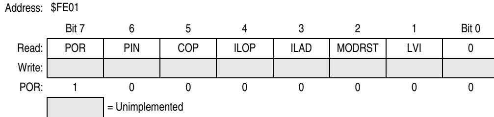
Figure 13-19. SIM Reset Status Register (SRSR)
