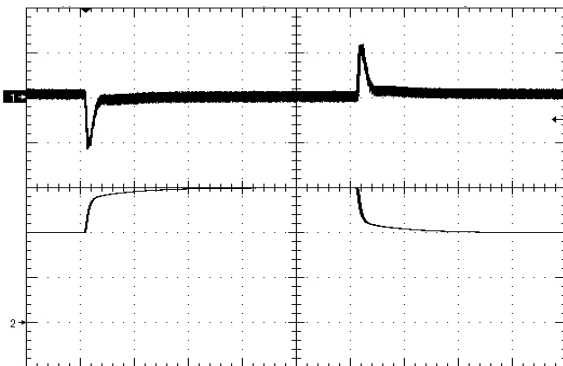
Figure 11. Load Transient Response (50mV/div), di/dt=0.1A/uS, 50% - 75% - 50% of full load, time scale: 200uS/div.
