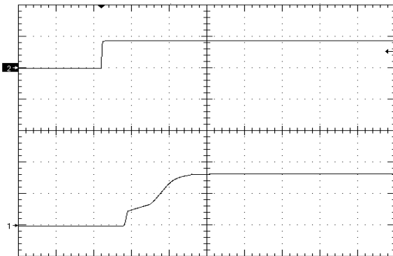
Figure 9. Startup Waveform via Enable Pin, time scale 10mS/div. Vin=Vin_nom, No Load (positive enable.) Ch1=2V/div,Ch2=5V/div
