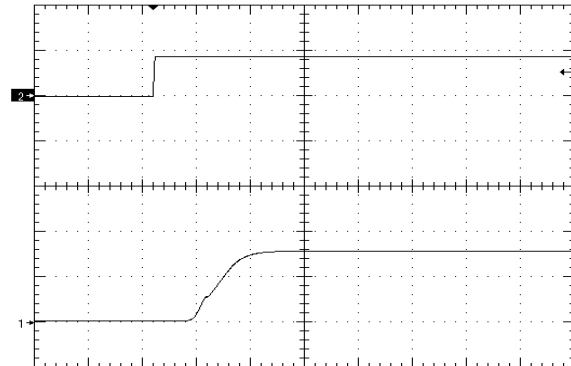
Figure 10. Startup Waveform via Enable Pin, time scale 10mS/div. Vin=Vin_nom, full load + 10000uF (pos. enable.) Ch1=2V/div,Ch2=5V/div
