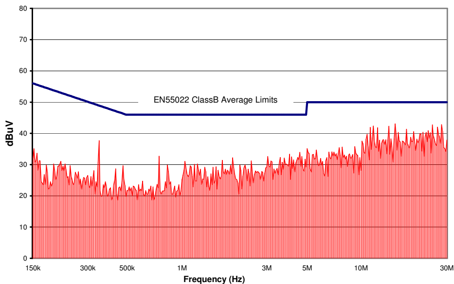
Figure 18. CPE20F18 Conducted Emissions using above specified input filter, Vin = 24V, Full Resistive Load
