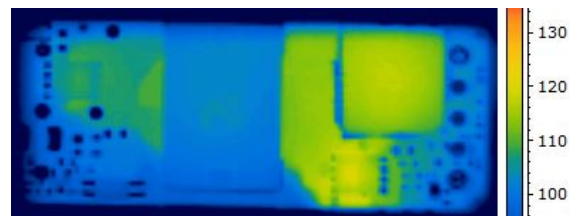
Thermal Image of module @ 24Vin, 200LFM & 70C
