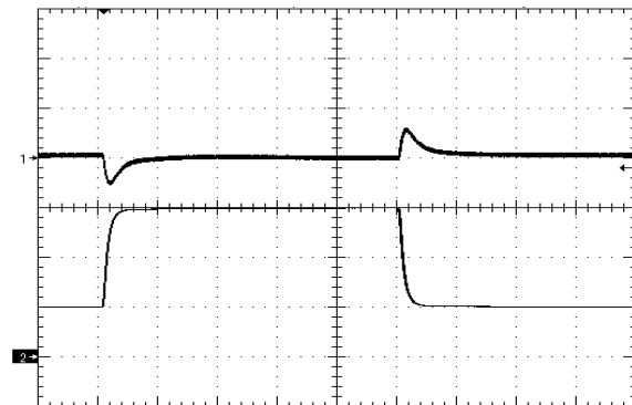
Figure 12. Load Transient Response (100mV/div), di/dt=0.2A/uS, 25% - 75% - 25% of full load, +4700uF, time scale: 200uS/div
