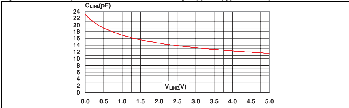
Figure 7. Line capacitance versus reverse voltage applied (typical value)
