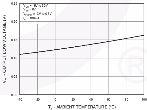
Fig. 6 Output Low Voltage vs. Ambient Temperature
