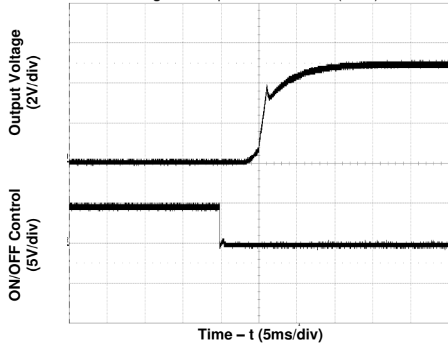
Figure 4. Start-Up Characteristic (typical Vin, full load)
