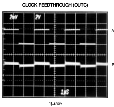
V SS = 0V, CS = HIGH A: SCLK, 333kHz, 0V TO 2.9V, 2V/div B: OUTC, 2mV/div
