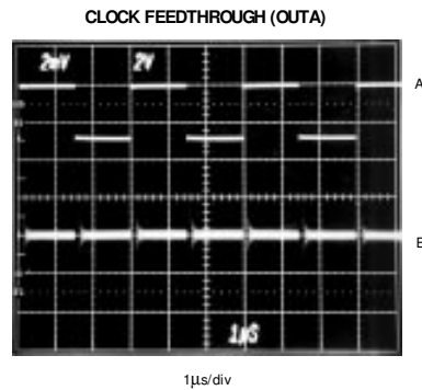
V SS = 0V, CS = HIGH A: SCLK, 333kHz, 0V TO 2.9V, 2V/div B: OUTA, 2mV/div
