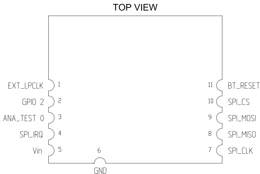
Figure 3. Pin connection
