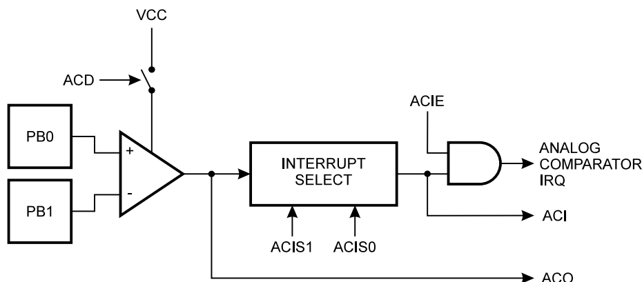
Figure 21. Analog Comparator Block Diagram
