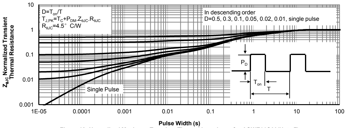
Figure 12: Normalized Maximum Transient Thermal Impedance for AOWF11C60(Note F)
