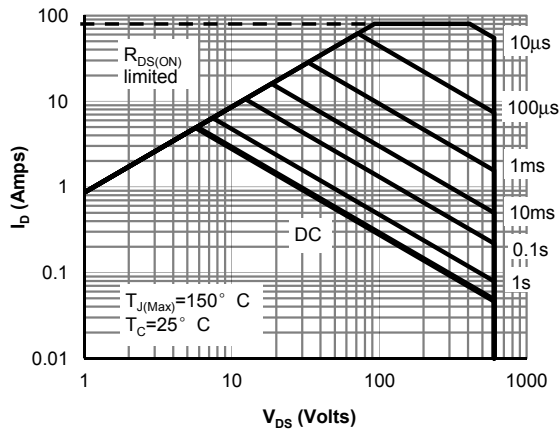
Figure 11: Maximum Forward Biased Safe Operating Area for AOWF11C60 (Note F)
