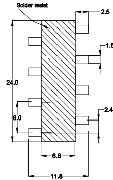
Recommended Pad Layout
