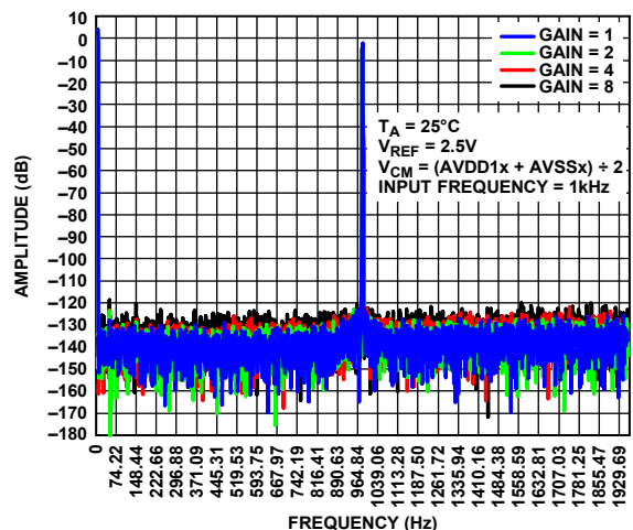
Figure 37. FFT Plot, Low Power Mode at 4 kSPS, Input Frequency ( f_{IN} ) = 1 kHz, Sinc3 Filter Enabled
