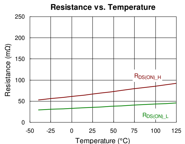
Figure 13. RT6274C/D R_{DS(ON)} vs. Temperature
