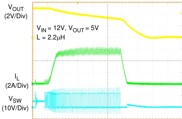
Time (10µs/Div)
