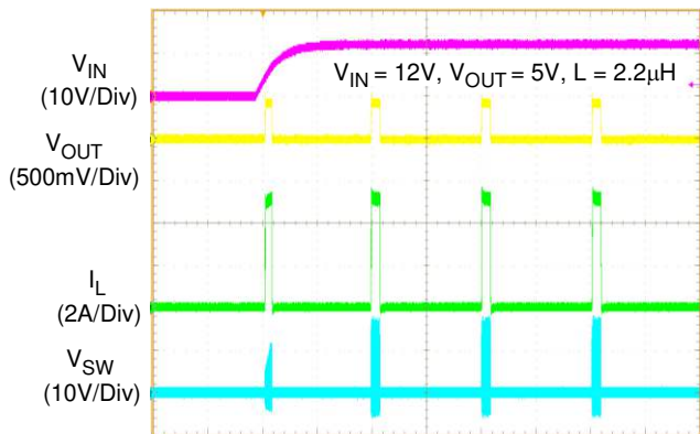
Time (10ms/Div)
