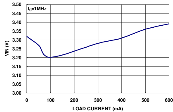
(a) V_{OUT}=3.3V
