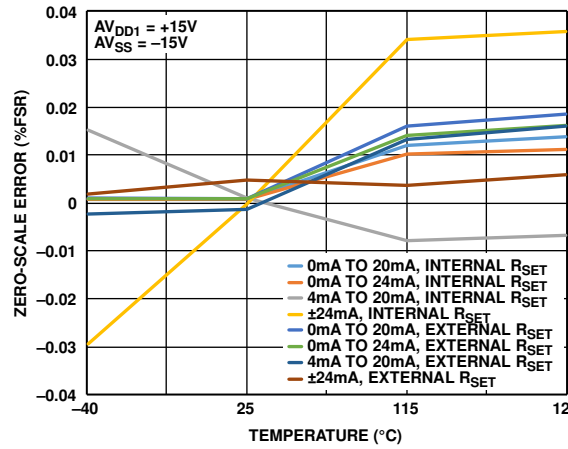
Figure 40. Zero-Scale Error vs. Temperature
