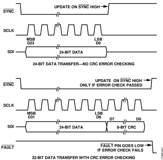
Figure 67. CRC Timing (Assume LDAC = 0)
