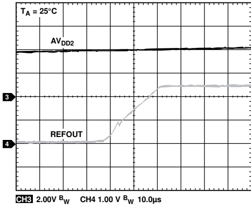
Figure 51. REFOUT Turn On Transient
