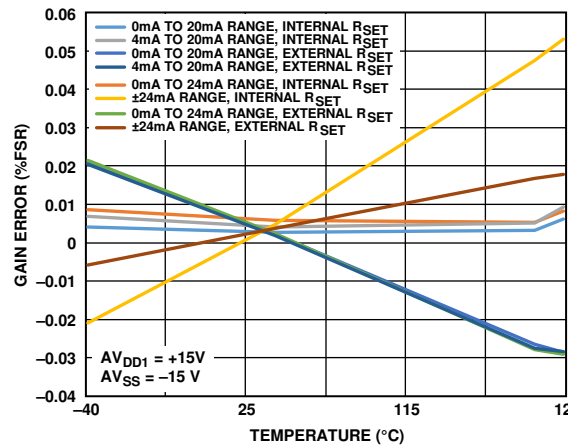
Figure 41. Gain Error vs. Temperature
