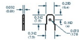
"Q" TERMINALS
