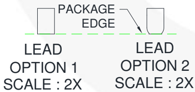
Figure 20. 12-Lead, Ultrathin Molded Leadless Package (UMLP)
