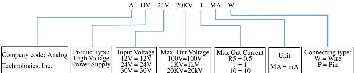
Figure 9. Naming Rules of AHV24V20KV1MAW
