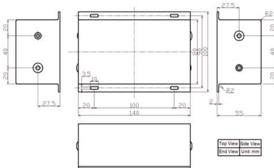
Figure 11. Dimensions for AHV24V20KV1MAW
